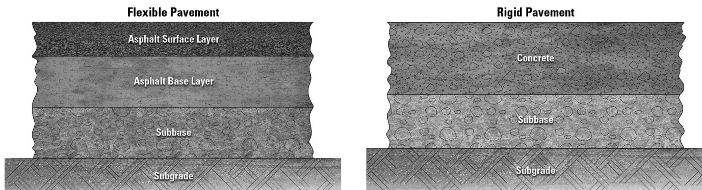
Figure 1.1. Pavement structure comparison
