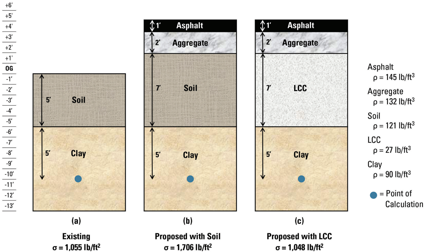
Figure 3.1. Net load design method for settlement reduction
