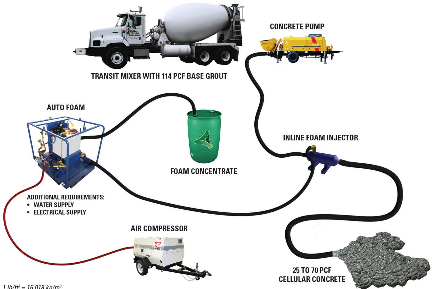
Figure 5.3. How foam is introduced into a ready-mixed concrete truck-based pumping system
